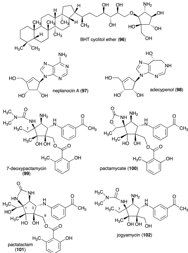
Fig. 20 Chemical structures of C-ribomimetics.
