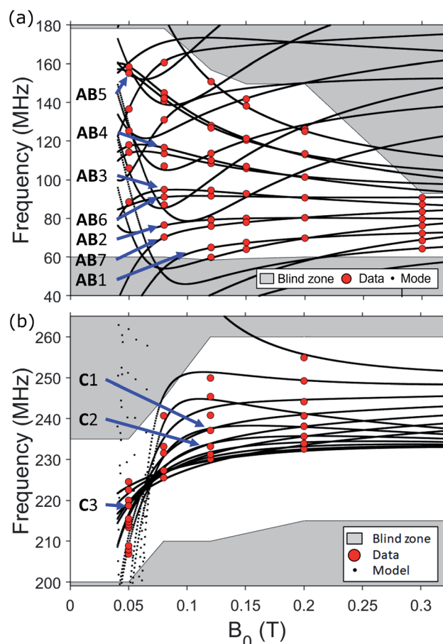
Fig. 3 Measured (red dots, T = 1.4\text{ K} ) and calculated (black lines) transition frequencies as a function of the applied field, applied along different directions: B_0 \in ab -plane (a) and B_0 \parallel c (b), with corresponding transitions labelled by "AB#" and "C#", respectively. Shaded grey areas are experimentally non-accessible or not explored.
