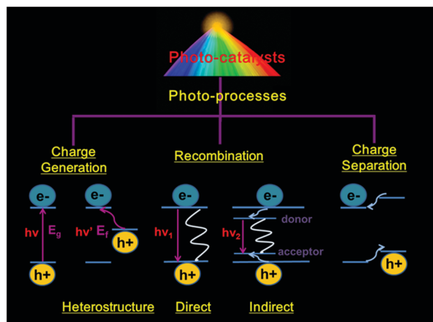
Fig. 2 Basic photo-process of photocatalysts. E_g : band gap of a semi-conductor and E_f : Fermi energy of the immobilized noble metal particles. After photo-excitation, radiative and non-radiative recombination can occur, as depicted by the straight and wavy lines, respectively.
