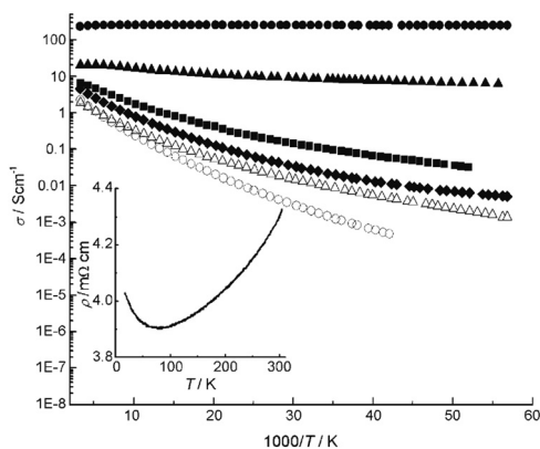
Fig. 9 Temperature dependence of electrical conductivity ( \sigma ) measured on polycrystalline samples of [\text{Au}(\text{dtdt})_2] ( \blacklozenge ), [\text{Au}(\alpha\text{-ttdt})_2] ( \blacksquare ), [\text{Ni}(\text{dtdt})_2] ( \bullet : oxidation by air exposure, \circ : iodine oxidation) and [\text{Ni}(\alpha\text{-ttdt})_2] ( \blacktriangle : oxidation by air exposure, \triangle : iodine oxidation). Inset: Temperature dependence of electrical resistivity ( \rho ) of [\text{Ni}(\text{dtdt})_2] , obtained by oxidation by air exposure. Reprinted with permission from ref. 61. Copyright © 2007 WILEY-VCH Verlag GmbH & Co. KGaA, Weinheim.
