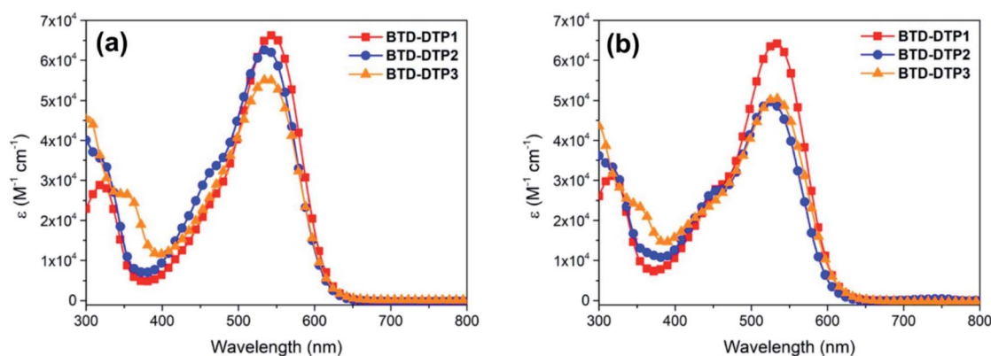
Fig. 4 UV-Vis absorption spectra of dyes BTD-DTP1–3 (a) in \text{CHCl}_3 solution, (b) in THF solution.
