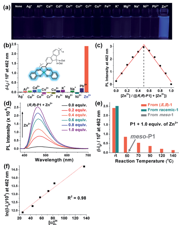
Fig. 6 Metal sensing experiments using P1 in THF : H 2 O = 9 : 1 (v/v) solution (10 \mu M) at 298 K. (a) Photoluminescence of (R,R) - P1 solution in the absence or presence of 1.0 equiv. of various metal cations under 365 nm UV irradiation. (b) Emission changes of (R,R) - P1 in the presence of 1.0 equiv. of various metal cations. (c) Job plot of (R,R) - P1 vs. Zn 2+ (total concentration = 20 \mu M). (d) Emission spectra of (R,R) - P1 with increasing amounts of Zn 2+ (0.0–1.0 equiv.). (e) Effect of polymerization temperature on the Zn 2+ sensing performance of P1 . (f) Correlation between fluorescence enhancement ( I - I_0 ) and optical rotation ( [\alpha]_D^{24} ) of P1 .
