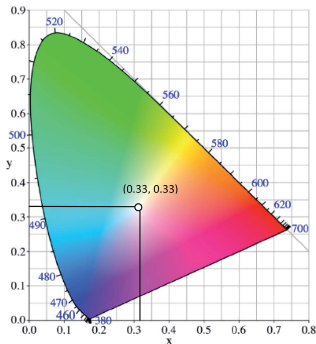
Fig. 1 The chromaticity coordinates ( x , y ) of pure white light, as given by the Commission Internationale d'Éclairage, is (0.33, 0.33). The figure was adapted from ref. 25 with accreditation given to Creative Commons Attribution 4.0 International Public License.
