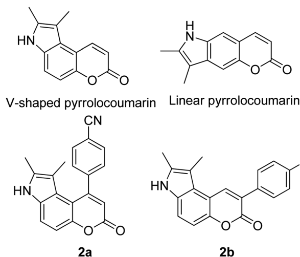
Fig. 4 Pyrrolocoumarin derivatives with chemical modification. The compounds are from ref. 43.
