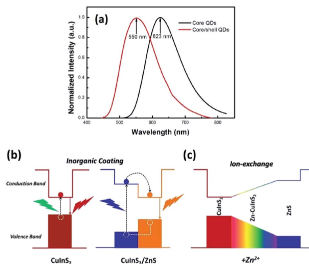
Fig. 8 (a) Normalized emission spectra of the CuInS 2 core QDs and CuInS 2 /ZnS core/shell QDs. (b) Photoluminescence emission mechanism of the CuInS 2 /ZnS core/shell QDs. (c) Schematic of the changes of the energy band gap with the addition of Zn 2+ . The figure was reproduced from ref. 61 with accreditation given to Creative Commons Attribution 4.0 International Public License.
