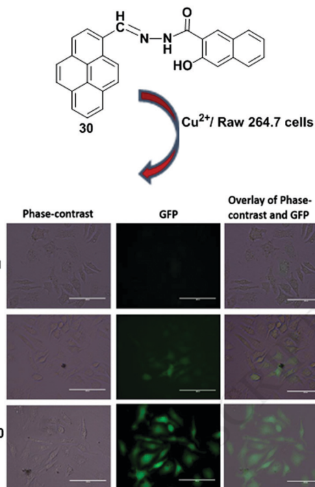
Fig. 26 Structure of ligand 30 . Fluorescence images of RAW 264.7 cells treated with chemosensor 30 and Cu 2+ ions. Phase-contrast (left); GFP image ( \lambda_{\text{ex}} = 393 nm) (middle); and overlay of phase-contrast and GFP (right). Reproduced from ref. 93 with permission from the Elsevier, copyright 2018.
