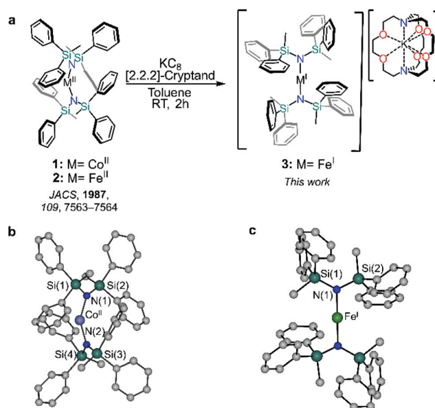
Fig. 1 Preparation of 1–3 and single crystal X-ray structure determinations of 1 and 3 . (a) Reaction scheme for the synthesis of [M\{\text{N}(\text{SiMePh}_2)_2\}_2] ( 1 , M = \text{Co}^{II} ; 2 , M = \text{Fe}^{II} ) and [K(2,2,2\text{-crypt})][Fe\{\text{N}(\text{SiMePh}_2)_2\}_2] ( 3 , M = \text{Fe}^I ). Solid-state molecular structures of 1 (b) and 3 (c) H atoms and [K(2,2,2\text{-cryptand})]^+ were omitted for clarity.
