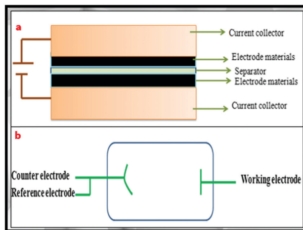
Fig. 18 Schematics presenting the cell connections of the two-electrode system.
