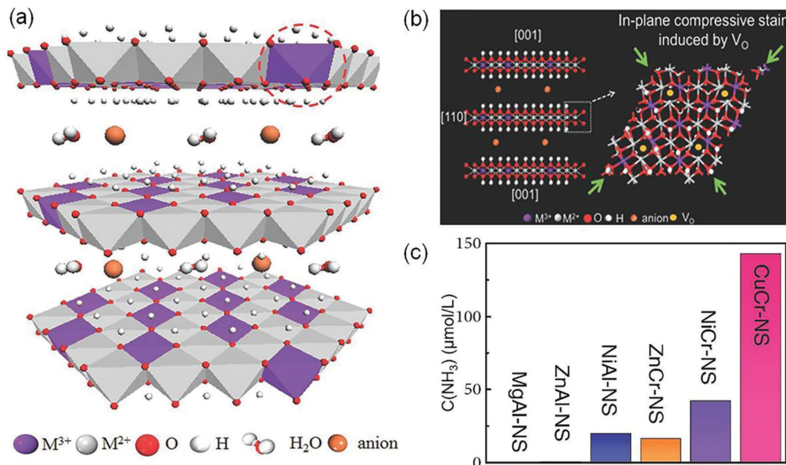
Fig. 4 (a) Schematic representation of the layered LDH structure with defective \text{MO}_6 octahedra. (b) Schematic of the in-plane biaxial compressive strain induced by \text{V}_o . (c) The yield of \text{NH}_3 over different LDH photocatalysts under visible-light illumination ( \lambda > 400 nm). Reproduced from ref. 34 with permission from Wiley-VCH.
