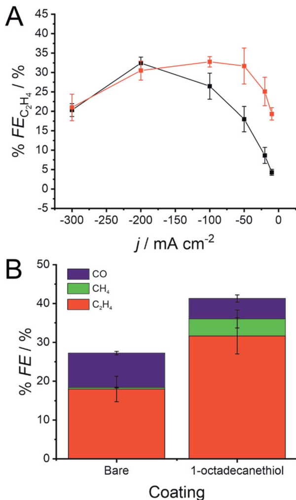
Fig. 4 (A) Faradaic efficiency for C_2H_4 formation ( \% FE_{C_2H_4} ) during galvanostatic CO_2 reduction at a 500 nm Cu GDE in 1 M KOH with (red) and without (black) a monolayer of 1-octadecanethiol to form a hydrophobic interface. (B) % FE for CO , CH_4 and C_2H_4 with and without the 1-octadecanethiol layer during galvanostatic CO_2 reduction at -50 \text{ mA cm}^{-2} using the same conditions as in (A). Error bars display one standard deviation ( n = 3 ).
