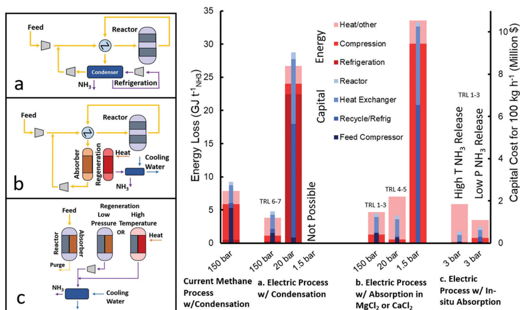
Fig. 5 Comparison of energy losses and capital requirements of different HB synthesis loop configurations taking 100 kg NH_3 h -1 as a basis production. In every case the reactor is at 400 °C. The high pressure processes have an operating pressure of 150 bar and either a condenser at −25 °C or an absorber at 300 °C, and approx. 140 bar after a 10 bar pressure drop. The medium pressure processes are at 20 bar, with a condenser at −33 °C or an absorber at 200 °C and 19 bar. The low pressure process is at 1.5 bar with an absorber temperature of 200 °C. The pressure of in situ absorption is 3 bar with a low temperature (250–300 °C) reactor. In situ absorbent can be regenerated by either high temperatures (350–400 °C) at >10 bar to subsequently condense ammonia or by release at atmospheric pressure and compressing ammonia before condensation (>10 bar). Calculations can be found in Section S.2 (ESI†) and are meant as estimates for comparison.
