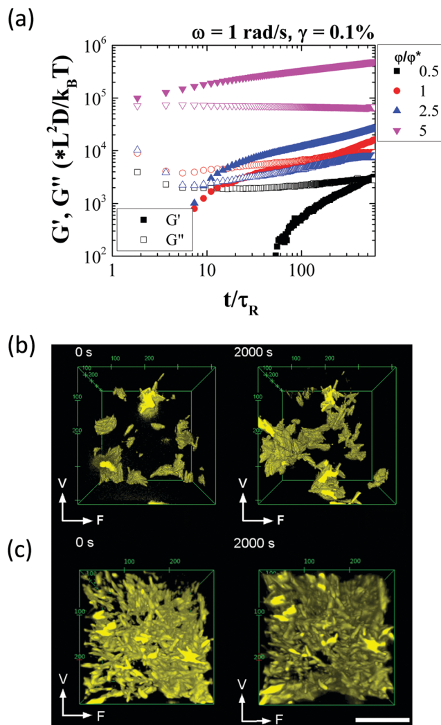
Fig. 3 (a) Time evolution of viscoelastic moduli for different rod volume fractions ( \phi/\phi^* = 0.5, 1, 2.5 and 5 ) at 1 \text{ rad s}^{-1} and 3D confocal micrograph ( 61 \times 61 \times 50 \text{ }\mu\text{m}^3 ) of the microstructure of the silica rod suspension at \phi/\phi^* = 1 (b) and \phi/\phi^* = 5 (c) captured immediately after rejuvenation [left], and 2000 s after rejuvenation [right] (scale bar: 20 \text{ }\mu\text{m} , V = vorticity, F = flow direction).
