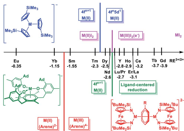
Chart 1 Scale of M 3+/2+ (M = rare earth metal) reduction potentials 28 and electron configurations of divalent rare earth metal complexes in different coordination environment: pink, M(II) 2 ; 29 blue, [K(crypt)](Cp' 3 M); 39 green, [K(crypt)](( Ad,Me ArO) 3 mes)M; 42 red, [(NN TBS )M] 2 (μ-biphenyl)[K(solvs)] 2 (this work).
