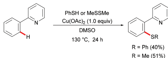
Scheme 37 \text{Cu}(\text{II}) -Catalysed C–H thiolations of arenes.
