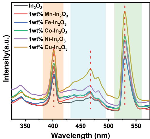
Fig. 6 Photoluminescence emission spectra of pure and transition metal ion-doped \text{In}_2\text{O}_3 . Three distinct regions of emission are marked with different colour shades.
