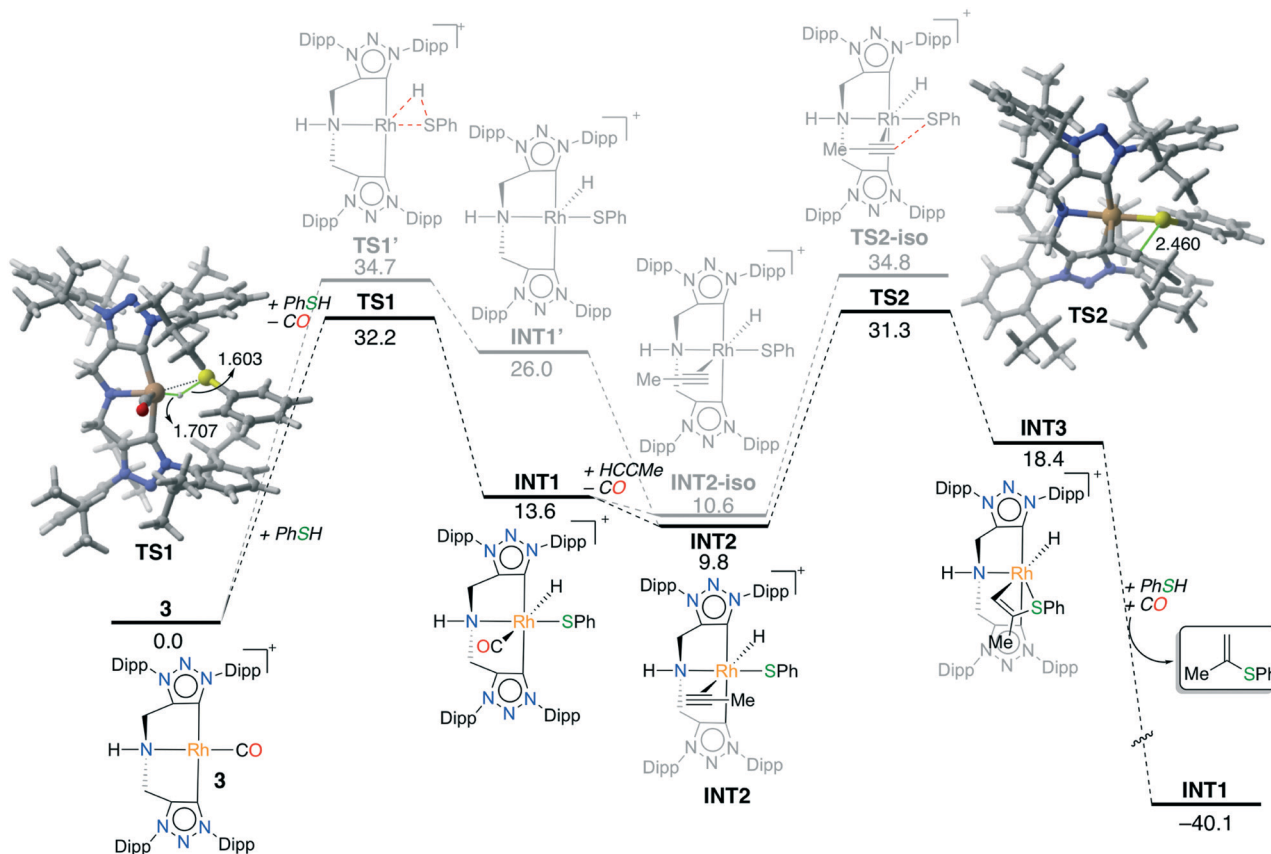
Fig. 2 Computed reaction profile for the reaction of PhSH and MeC≡CH catalysed by complex 3. Relative free energies (within parentheses, \Delta G_{298} , computed at 298 K) are given in kcal mol -1 whereas bond distances are given in Ångströms. All data have been computed at the PCM(benzene)-B3LYP-D3/def2-SVP level.
