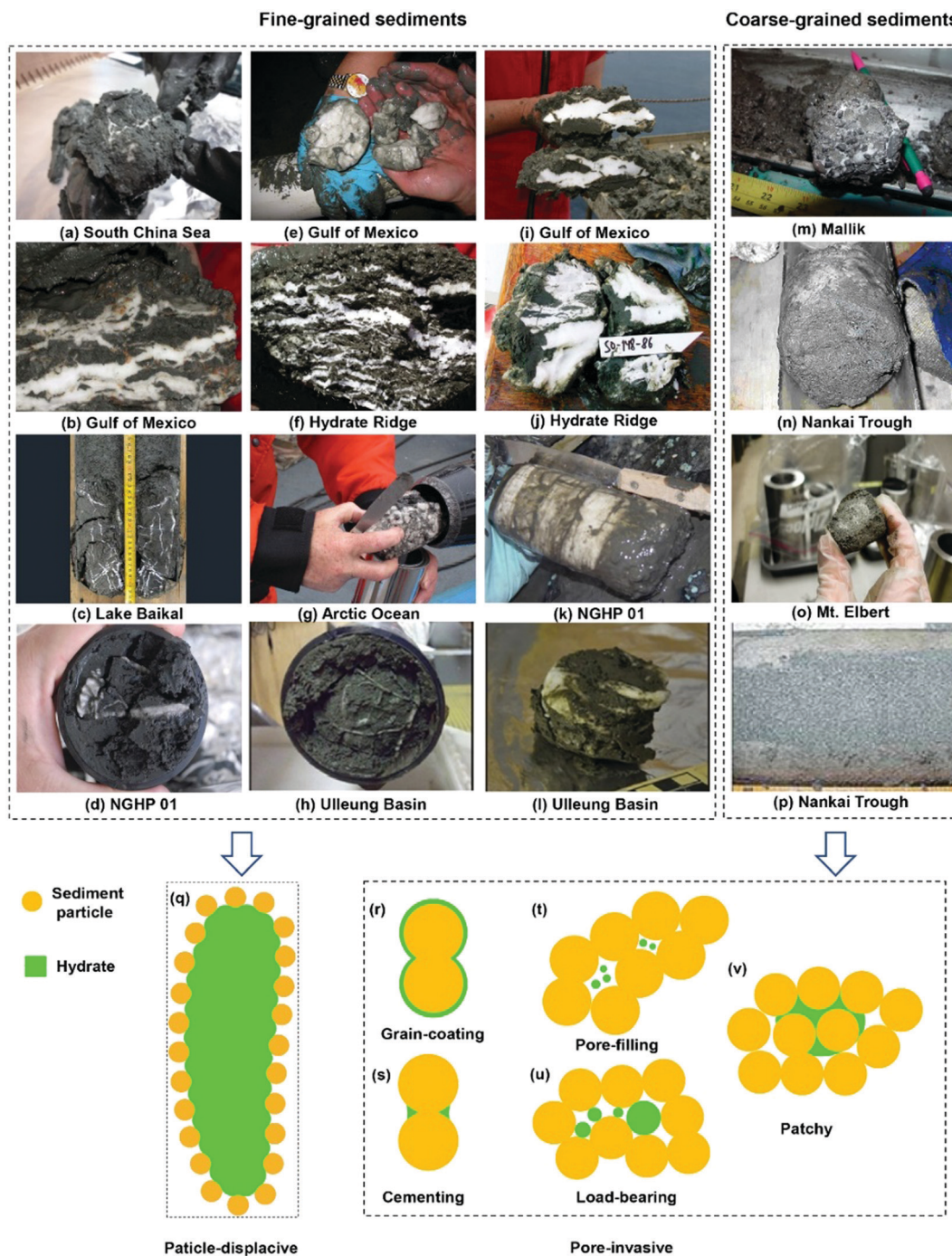
Fig. 8 Core-scale hydrate morphology in HBS samples and conceptual pore-scale habits for fine-grained and coarse-grained sediments (reprinted with permission from Ren et al. , 403 Copyright 2020 Elsevier Ltd).
