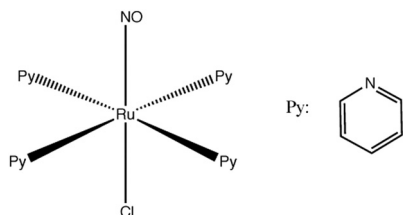
Scheme 3 Schematic structure of [\text{RuCl}(\text{NO})(\text{py})_4]^{2+} .
