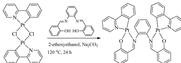
Scheme 2 Synthesis of binuclear [(C^N)Pt(\mu-Salen)Pt(C^N)] complexes.
