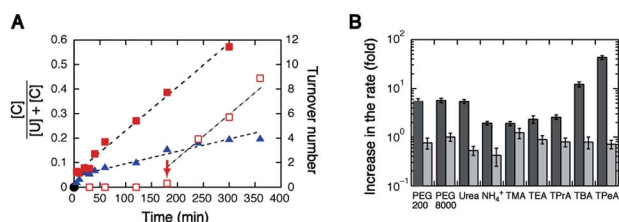
Fig. 2 (A) Kinetic traces for the substrate cleavage under the multiple-turnover condition in the presence of 100 mM TBA (blue triangles) or 100 mM TPeA (red closed squares). In one case, 100 mM TPeA was added 3 h after the addition of \text{MgCl}_2 (indicated by an arrow) to initiate substrate cleavage, represented by open squares. (B) Relative rate increases (relative to control) of multiple-turnover cleavage (black) and single-turnover cleavage (gray) by the addition of 20% PEGs, 2 M urea, 100 mM \text{NH}_4^+ , or 100 mM tetraalkylammonium ions.
