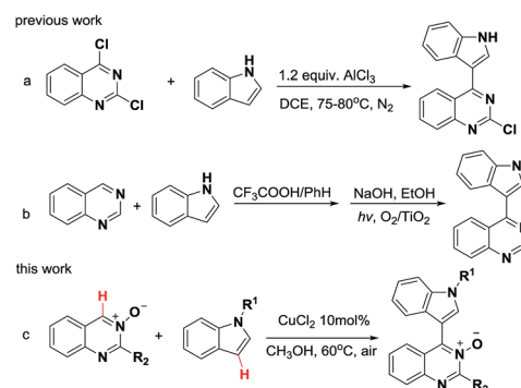
Scheme 1 Typical strategies for the synthesis of 4-(indole-3-yl)quinazolines.
