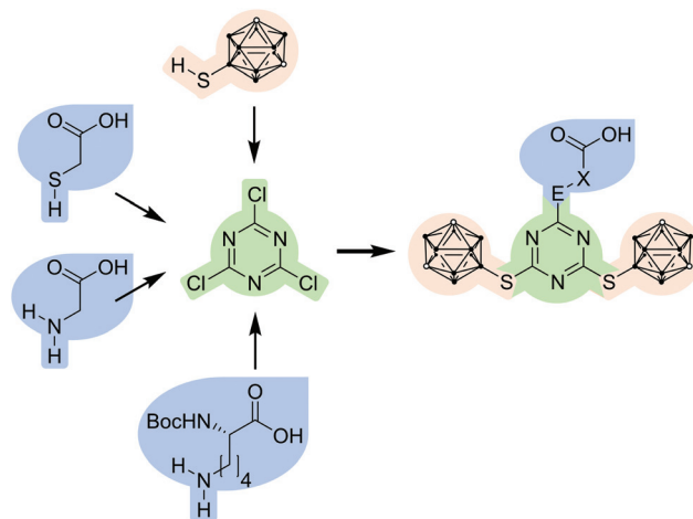
Fig. 1 Combination of a carborane-based building block (pale red) and carboxylic acid derivatives (blue) with cyanuric chloride (green) as a central branching unit and nucleophilic side chains (E = NH or S; X = CH 2 or (CH 2 ) 4 CHNH 2 (Boc = tert -butoxycarbonyl)).
