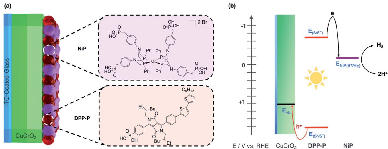
Fig. 1 (a) Dye (DPP-P) and catalyst (NiP) co-immobilised on the \text{CuCrO}_2 electrode with their molecular structures. (b) Energy diagram showing movement of electrons with black and holes with red arrows. S represents the dye sensitizer where E_{(S^*/S^-)} is the ground state reduction potential and E_{(S/S^*)} is the reduction potential in the excited state. E_{\text{NiP}(H^+/H_2)} is the catalytic onset potential for NiP and E_{\text{vb}} is the \text{CuCrO}_2 valence band potential.
