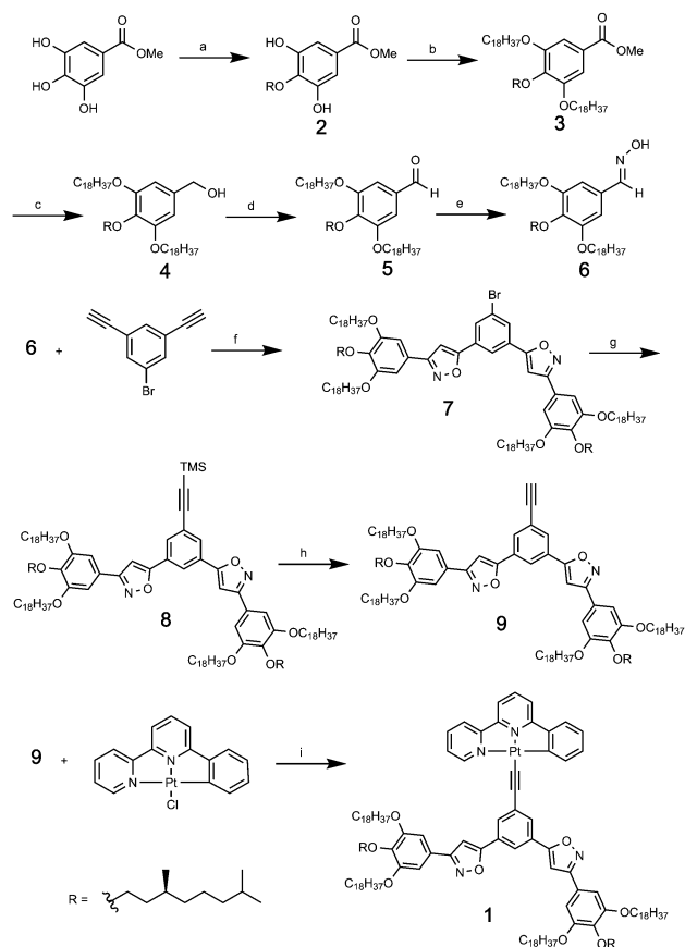
Scheme 1 Synthetic procedure for compound 1 . (a) ( S )-1-Bromo-3,7-dimethyloctane, K 2 CO 3 , dimethylformamide (DMF), 50%. (b) 1-Bromooctadecane, Cs 2 CO 3 , 2-butanone, 60%. (c) LiAlH 4 , tetrahydrofuran (THF), 97%. (d) MnO 2 , CH 2 Cl 2 , 98%. (e) NH 2 OH·HCl, NaOH, THF, H 2 O, 95%. (f) t BuOCl, NaI, 2,6-lutidine, 1,4-dioxane, 61%. (g) Trimethylsilyl acetylene, PdCl 2 (PPh 3 ) 2 , CuI, i Pr 2 NH, THF, 74%. (h) Tetrabutylammonium fluoride (TBAF), THF, 83%. (i) Triethylamine, CuI, CH 2 Cl 2 , 42%.
