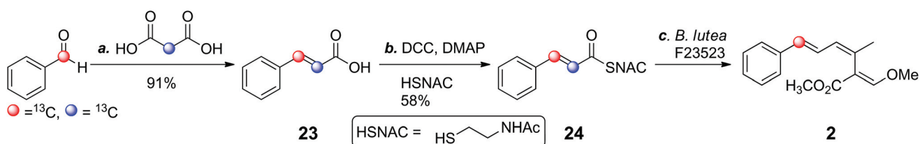
Scheme 1 (a) Incorporation of ^2\text{H} and ^{13}\text{C} -labelled precursors into strobilurin A 2 in S. tenacellus and B. lutea . (b) Proposed assembly and rearrangement of strobilurin tetraketide.
