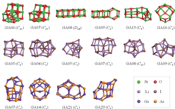
Fig. 9 Ball and stick models of (XY)_{12} IP-LM configurations obtained by the genetic algorithm that were missing from the IP-LM found using the data-mining approach. The colour scheme is shown in the lower right hand panel and is the same as that employed in previous figures. The numbers in the GA** labels indicate the rank found for the nano-cluster, where 01 indicates the IP-GM, whereas in the previous labels, DM**, they indicate the rank before the missing IP-LM were found using the GA.
