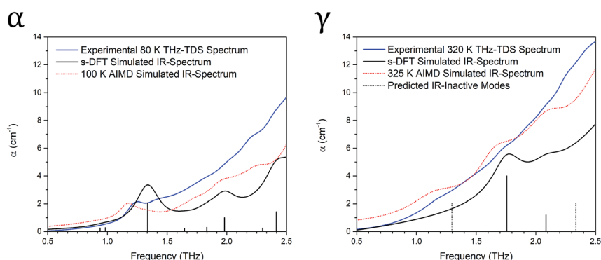
Fig. 5 Experimental THz-TDS spectra (blue) and s-DFT simulated IR spectra (black) for both PCB solids. The \alpha -PCB spectrum (80 K) is predicted to have a number of IR-active modes which primarily correspond to hindered-rotational motions of the individual molecules within the solid. The \gamma -form contains fewer IR-active modes (due to the smaller static unit cell compared to the \alpha -form), however there are additional IR-inactive modes (dotted lines) predicted that might be activated in the experimental disordered structure. In both panels, the simulated AIMD spectra are also shown as dotted red lines, and are in good general agreement with the experimental spectra. Note that the experimental spectra have been offset by +1.5 \text{ cm}^{-1} for clarity.
