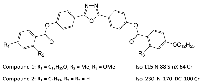
Fig. 1 Molecular structure and phase transitions for compounds 1 and 2 where the transition temperatures are recorded in °C, and Iso = isotropic phase, N = nematic phase, SmX = smectic phase of unknown type, DC = dark conglomerate phase and Cr = crystalline phase.
