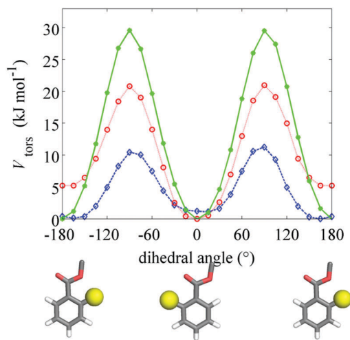
Fig. 6 Torsional potential, V_{\text{tors}} , as a function of the C–C–C=O dihedral angle, calculated for phenyl benzoate with different substituents in the ortho position of the benzoate ring: H (green solid line with stars), \text{CH}_3 (red dotted line with circles), \text{OCH}_3 (blue dashed line with diamonds). The chemical structures on the bottom show the conformation of the benzoate group in correspondence of the minima of the torsional potential. The yellow sphere is in the position of the substituent.
