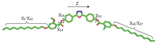
Fig. 3 Molecular structure of compound 1 without hydrogen atoms. Arrows show the dihedral ( \chi_i ) allowed to rotate in the Monte Carlo conformation sampling. The molecular frame \{x, y, z\} has the z axis passing through the carbon atoms of the oxadiazole ring and y perpendicular to the plane of the ring.
