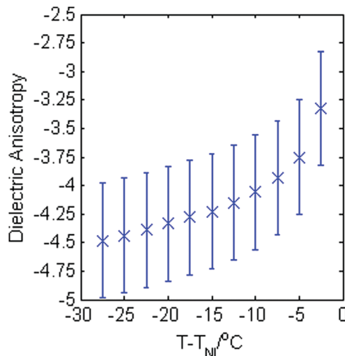
Fig. 4 Dielectric anisotropy as a function of T - T_{NI} for compound 1 .
