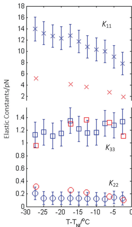
Fig. 5 The splay, K_{11} (crosses), twist, K_{22} (circles) and bend, K_{33} (squares) elastic constants as a function of T - T_{NI} for compound 1 . The experimental data are represented by the blue data points and the calculated data by the red data points. Note the break in the axis and the change in scale to make visible the very low twist and bend elastic constants.
