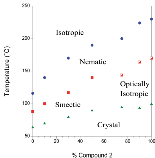
Fig. 2 The phase diagram of mixtures of compound 2 in compound 1 . The blue points mark the isotropic to nematic transition, the solid red data points represent the transition from the nematic to an unknown smectic (probably smectic C) phase, while the half-filled red data points represent the transition from a nematic to an optically isotropic phase. In the case of pure compound 2 , the optically isotropic phase is the dark conglomerate (DC phase). The green data points mark the mesophase to crystal transition. The POM and DSC traces are available from the linked data repository, https://doi.org/10.5518/207 .
