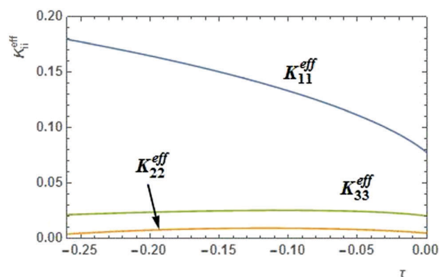
Fig. 10 Theoretical profiles of the splay, twist and bend elastic constants in compound 1 , calculated as functions of the reduced temperature taking into account the effect of chiral fluctuations and polar interactions of the bent-core molecules. The effective splay and bend constants were calculated using eqn (57)–(59) from ref. 3 for \epsilon = 75 , l = 2.5d , \alpha = 30^\circ and \psi = 0.009 (all parameters in this caption are as defined in ref. 3). The twist elastic constant for a bent-core molecule with the same opening angle ( 120^\circ ) is obtained from eqn (6) with A = 1/120 and t_c = 0.05 .
