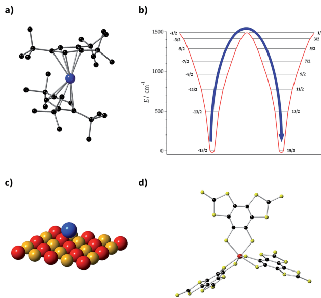
Fig. 5 (a) Molecular structure of [\text{Dy}(\text{Cp}^{\text{tBu}})_2]^+ , where \text{Cp}^{\text{tBu}} = \{\text{C}_5\text{H}_2\text{tBu}_3\text{-}1,2,4\} and \text{tBu} = \text{C}(\text{CH}_3)_3 . H atoms are omitted for clarity. Dy: blue and C: black. (b) Energy levels and M_J projections of [\text{Dy}(\text{Cp}^{\text{tBu}})_2]^+ , determined by CASSCF-SO calculations. (c) Ho atom on a MgO monolayer. Mg: yellow and O: red. (d) Molecular structure of [\text{V}(\text{C}_8\text{S}_8)_3]^{2-} . V: red, C: black, and S: yellow.
