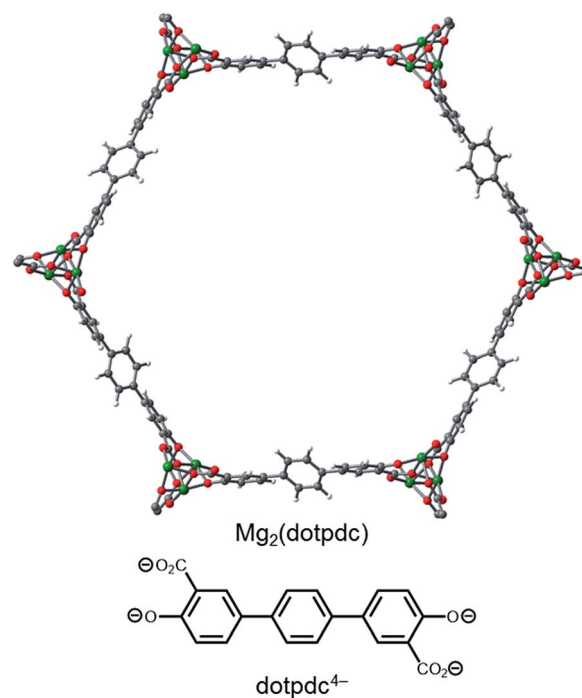
Fig. 7 Structure of the organic linker dotpdc^{4-} = 4,4'' -oxido-[ 1,1':4',1'' -terphenyl]- 3,3'' -dicarboxylate and a model of the hexagonal pore of Mg_2(dotpdc) . Green, grey, red, and white spheres correspond to Mg, C, O, and H, respectively.
