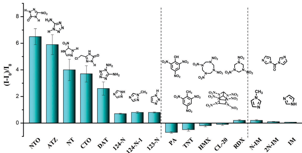
Fig. 3 Fluorescence enhancement ((I - I_0)/I_0) of E,E -HPB-ID by different analytes ( M_{E,E-HPB-ID} : M_{analytes} = 1 : 2 ) in the 90% water fraction in THF/water mixtures. [E,E-HPB-ID] = 1 \times 10^{-4} \text{ mol L}^{-1} .
