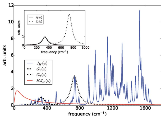
Fig. 2 Photosystem II reaction centre spectral densities. The components of the spectral densities used in the PSIIRC photocell model. Mode parameters of the structured component J_{\text{M}}(\omega) are shown in Table S1.† The Drude part J_{\text{D}}(\omega) is scaled relative to the high energy parts for clarity. The inset shows the spectral densities J_1(\omega) and J_2(\omega) which are used to approximate the full spectral density.
