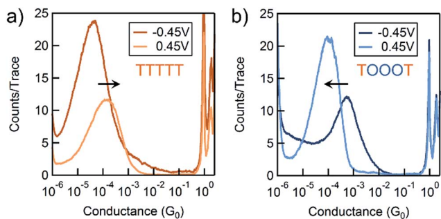
Fig. 2 Conductance histograms at two tip-biases for (a) TTTTT and (b) TOOOT respectively measured in propylene carbonate. The arrows indicate increasingly positive biases.
