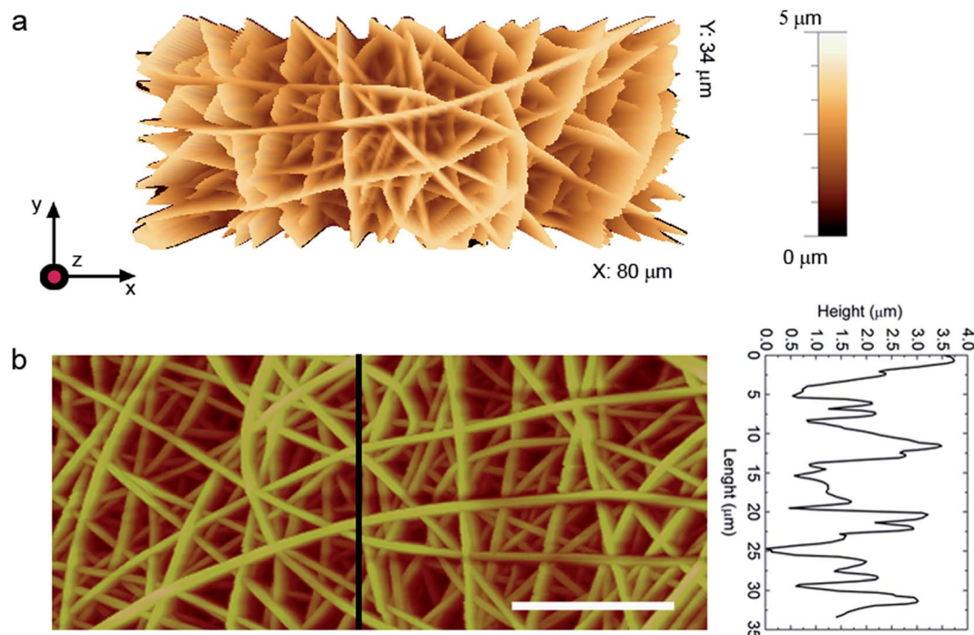
Fig. 3 AFM topographic micrograph of a fiber mat (2-Rg). (a) 3D view. (b) 2D view. Scale bar: 20 \mu\text{m} . Vertical scale: 5 \mu\text{m} . The height profile is taken along the line highlighted in the planar view.
