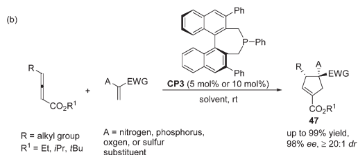
Scheme 15 The catalytic asymmetric Lu's [3 + 2] cycloadditions reported by Fu's group.
