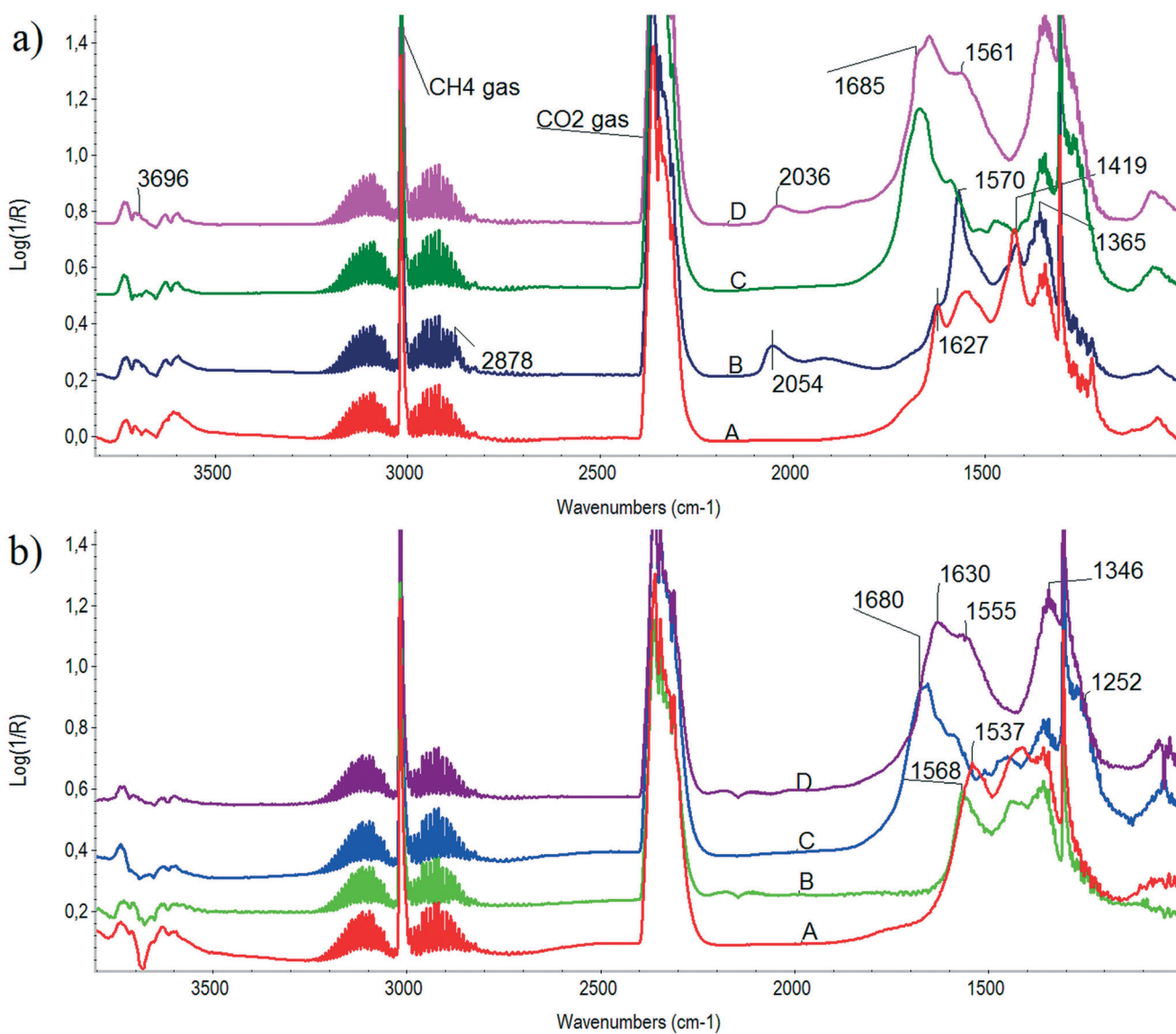
Fig. 4 DRIFTS spectra obtained in the presence of CH 4 :CO 2 = 70:30 DRM flow at (a) 300 °C and (b) 500 °C. Curve A: ZrO 2 support, B: Ni/ZrO 2 , C: Na-ZrO 2 support, D: Na-Ni/ZrO 2 .
