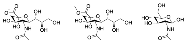
Fig. 9 Structures of sialic acid (left), the corresponding methyl ester (centre) and N -acetyl- D -glucosamine (right).
