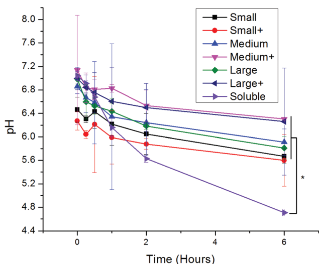
Fig. 3 Log-mean pH of red/green PNP upon incubation with DCs for various times following a two-hour pulse of PNP. Differences in log-mean pH were significant ( p < 0.05 ) between soluble OVA and all PNP except small coated (red circles). Each point is shows an average and standard deviation of three independent replicates ( n = 3 ).
