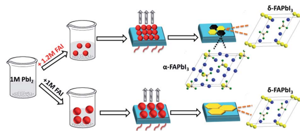
Fig. 5 Schematic view of the possible crystal growth process of FAPbI 3 films via controllable precursors. The unit cell of FAPbI 3 : yellow: Pb; gray: I; green: N; blue: F.
