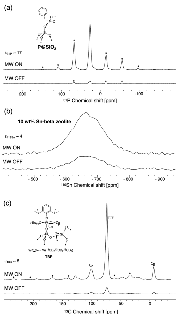
Fig. 1 DNP (a) ^{31P} CP Hahn-echo spectra of P@SiO 2 , (b) ^{119Sn} reconstructed CP-CPMG spectra of 10 wt% Sn-beta zeolite and (c) ^{13C} CP spectra of a single-site tungsten TBP metallacycle with microwaves on (top) and off (bottom). All samples were impregnated with a 16 mM solution of PyPolB-D2[G3] in TCE. Asterisks mark spinning side bands. NMR acquisition details are given in the ESI.†
