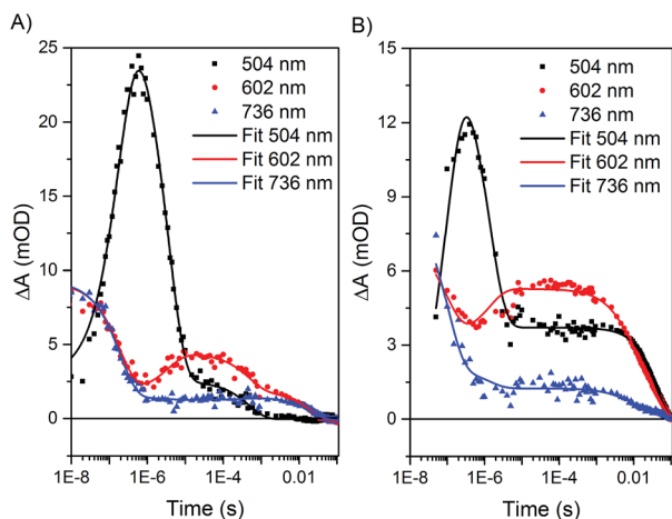
Fig. 6 Kinetic fits of transient optical kinetic data for the (A) Ru–ApoFld–CoBF 2 and (B) Ru–Fd–CoBF 2 biohybrids with 200 mM sodium ascorbate using a global kinetic fitting routine in Origin Pro 9.1. The data sets were fit with four-exponential decay functions from 10–50 ns to 100 ms.
