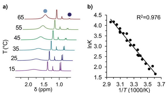
Fig. 2 (a) Variable temperature 1 H-NMR spectra of the equilibrium between t Bu-1· (●) and t Bu-1 2 (●) and (b) the corresponding van't Hoff plot (see ESI† for complete spectra).
