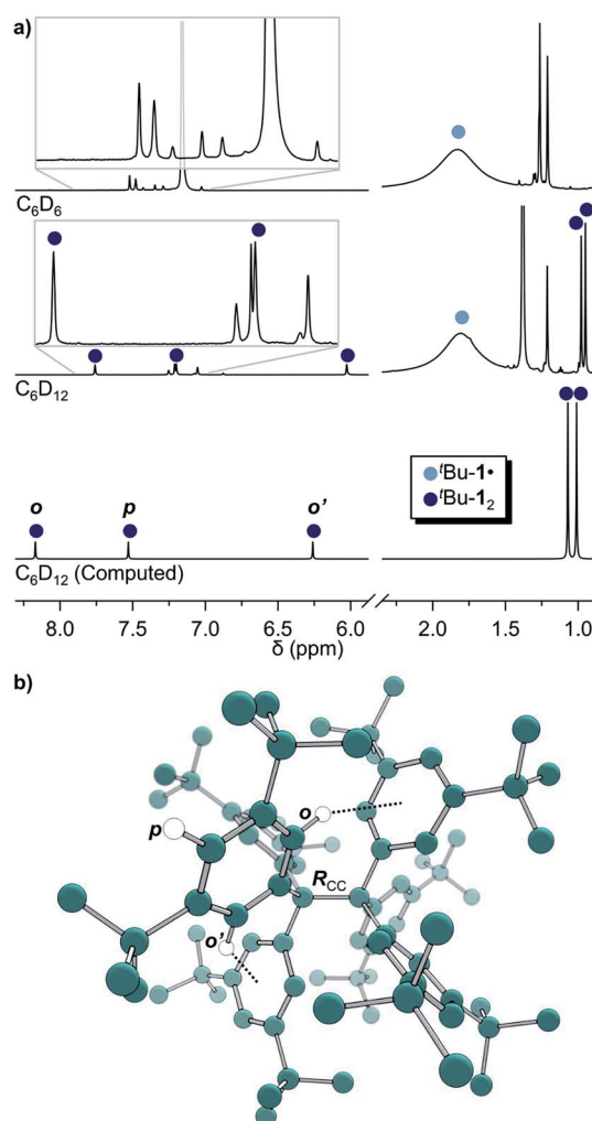
Fig. 1 (a) 1 H-NMR of t Bu-1· in benzene- d 6 (top) in equilibrium with t Bu-1 2 in cyclohexane- d 12 (middle) and the computed spectrum (iii) of t Bu-1 2 (bottom); see ESI† for full spectra. (b) The structure of t Bu-1 2 for NMR computations. R CC : exp. 4 1.67(3) Å, comp. 1.662 Å. (iii) (B3LYP-D3(BJ)/6-31G(d,p)/C-PCM:cyclohexane).
