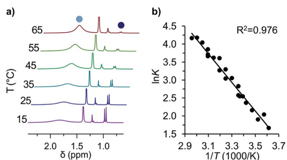
Fig. 2 (a) Variable temperature 1 H-NMR spectra of the equilibrium between t Bu-1· (●) and t Bu-1 2 (●) and (b) the corresponding van't Hoff plot (see ESI† for complete spectra).
