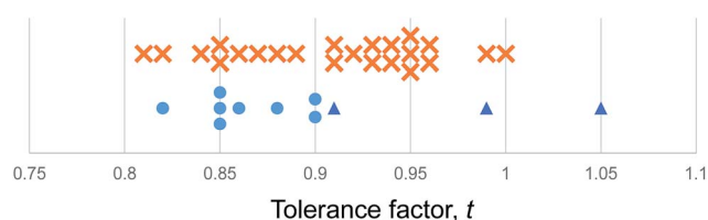
Fig. 1 The tolerance factors of \text{ABi}_3 compounds. Blue dots represent inorganic \text{ABi}_3 compounds that form perovskites at room temperature and pressure. Red crosses represent inorganic \text{ABi}_3 compounds that do not form perovskites. Blue triangles show hybrid \text{APbI}_3 and \text{ASnI}_3 compounds that form in the perovskite structure, using the methodology of Cheetham et al. to estimate molecular ion radii. 26,27 There is no boundary on the tolerance factor scale that separates perovskites from non-perovskites.
