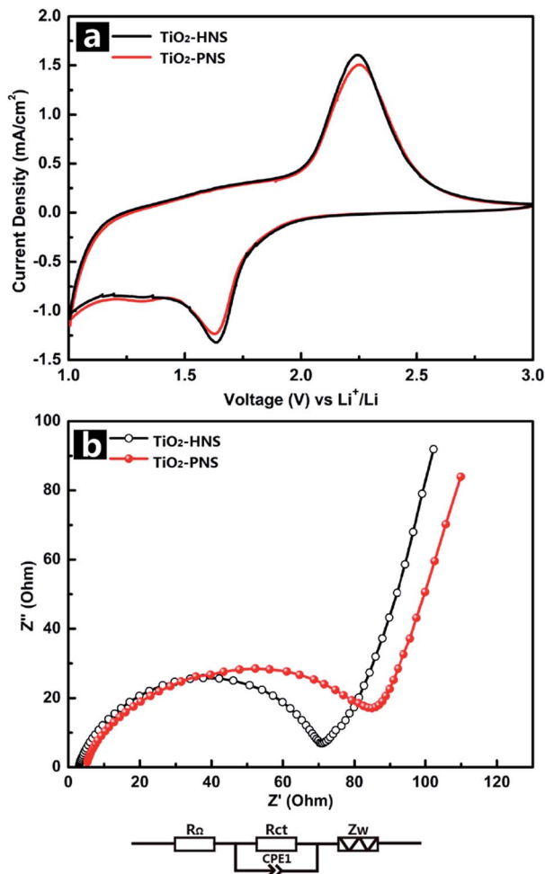
Fig. 4 (a) Cyclic voltammograms profiles of the \text{TiO}_2 -HNSs and \text{TiO}_2 -PNSs at a scan rate of 1 \text{ mV s}^{-1} between 1.0 V and 3.0 V for the first cycle, and (b) electrochemical impedance spectra (EIS) of the \text{TiO}_2 -HNSs and \text{TiO}_2 -PNSs ( R_n : external resistance, R_{ct} : charge transfer resistance, CPE1: constant phase element, Z_w : Warburg impedance).
