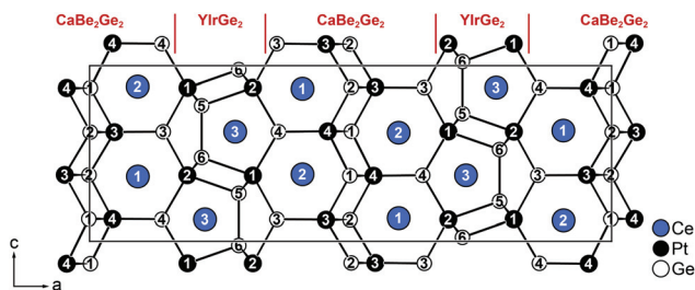
Fig. 3 Extended unit cell of the commensurate supercell structure ( Pnma , a = 2618.26(14) , b = 441.33(2) and c = 882.34(2) pm) of Ce_3Pt_4Ge_6 . The YrGe_2 and CaBe_2Ge_2 type parts are labelled. Ce atoms are depicted as blue, Pt atoms as black and Ge atoms as open white circles.
