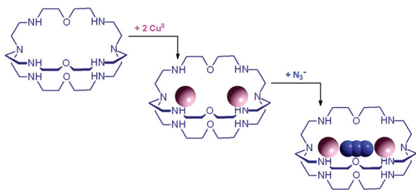
Fig. 1 Cascade process for the consecutive inclusion of two \text{Cu}^{\text{II}} ions, then of one azide anion into the bistrin cryptand 2 , to form the ternary dimetallic complex [\text{Cu}^{\text{II}}_2(2)(\text{N}_3)]^{3+} . Each terminal atom of the ambidentate anion establishes a coordinative interaction with a coordinatively unsaturated \text{Cu}^{\text{II}} centre bound to each tren subunit.
