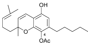
15 4-Acetoxycannabichromene [37]
