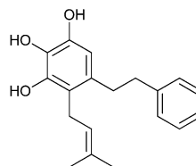
83 [178]
