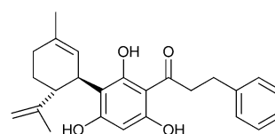
Linderatin 80 [197]
