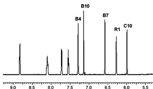
Fig. 3 ^1\text{H} NMR spectrum of [(\text{Re})-(\text{Co})-\text{CN}-(\text{cis-PtCl}(\text{NH}_3)_2)]^+ ( 2 ).
